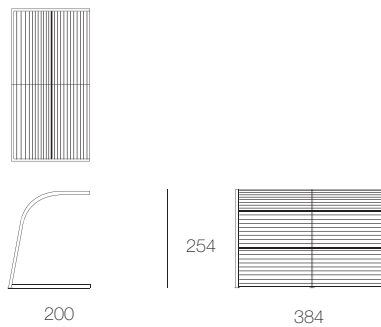
CA01FBH Modulo Veranda in wood with base, high uprights
