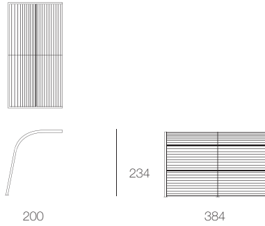
CA01FH Modulo Veranda in wood without base, high uprights
