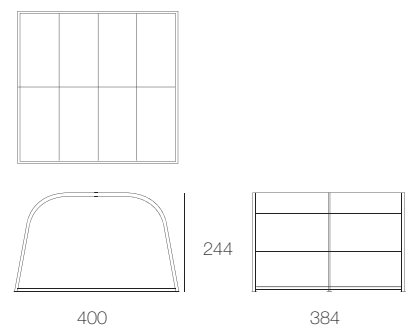
CA02ATBH Modulo Tunnel in fabric with base, high uprights
