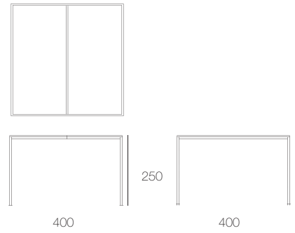
CA01AH structure without base
