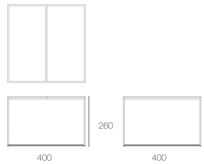
CA01ABH structure with base
