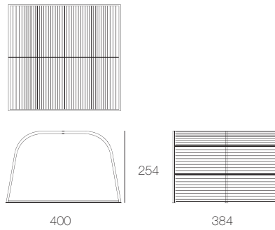
CA02ABH Modulo Tunnel in wood with base, high uprights
