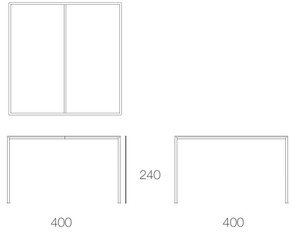
CA01AH structure without base
