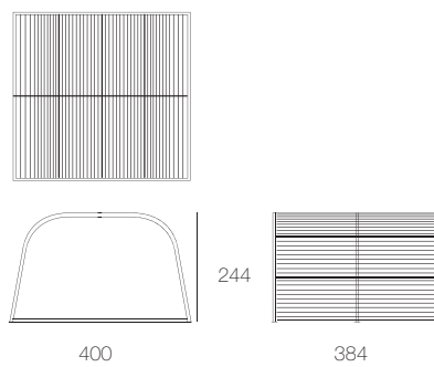
CA02ABH Modulo Tunnel in wood with base, high uprights
