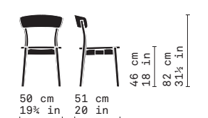
Trix 11 sedia dining /dining chair
