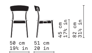
Trix 11/L sedia dining /dining chair
